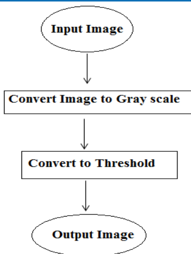
Fig 3 step pre-processing
