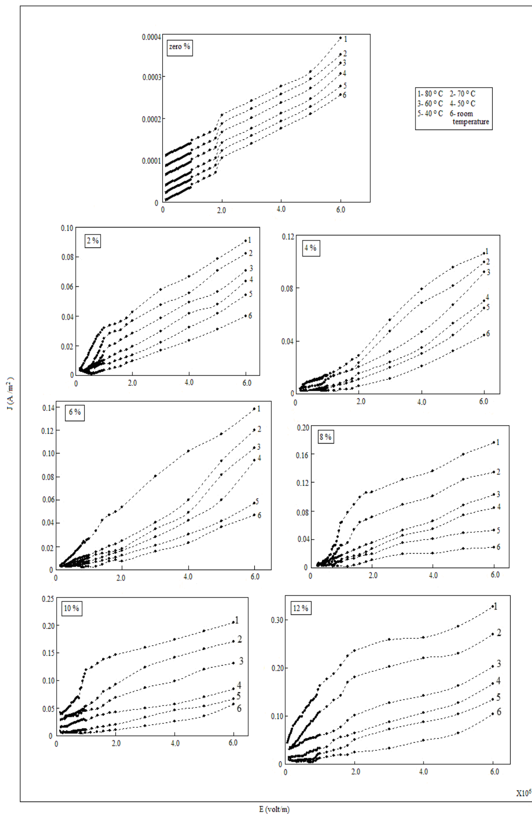
Fig 6 Variation of J with E for PVA/PEG/Ag nanocomposite samples with different concentration of Ag nano-particles and different temperatures.
