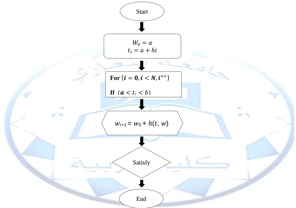
Figure 4 Euler algorithm to solve it by Java
