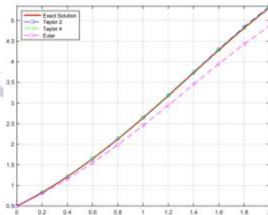
Figure 3 the exact solution, Euler, the second order and the 4th-order of Taylor method
