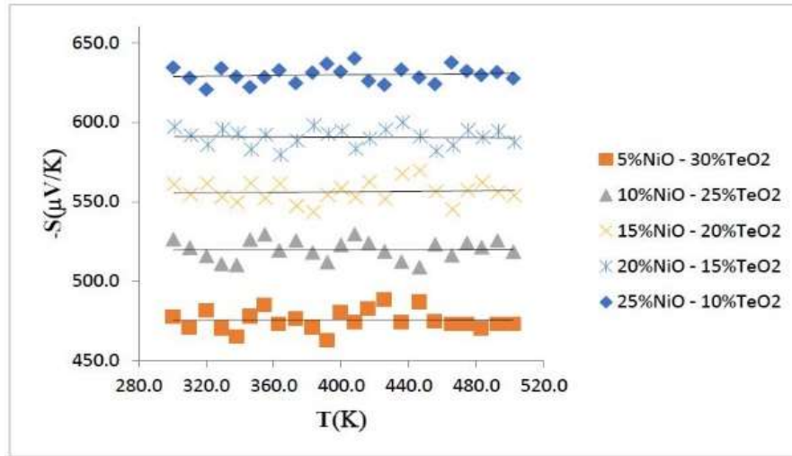
Fig. 4: Seebeck Coefficient(S) vs temperature T for five NiO glass composition.
