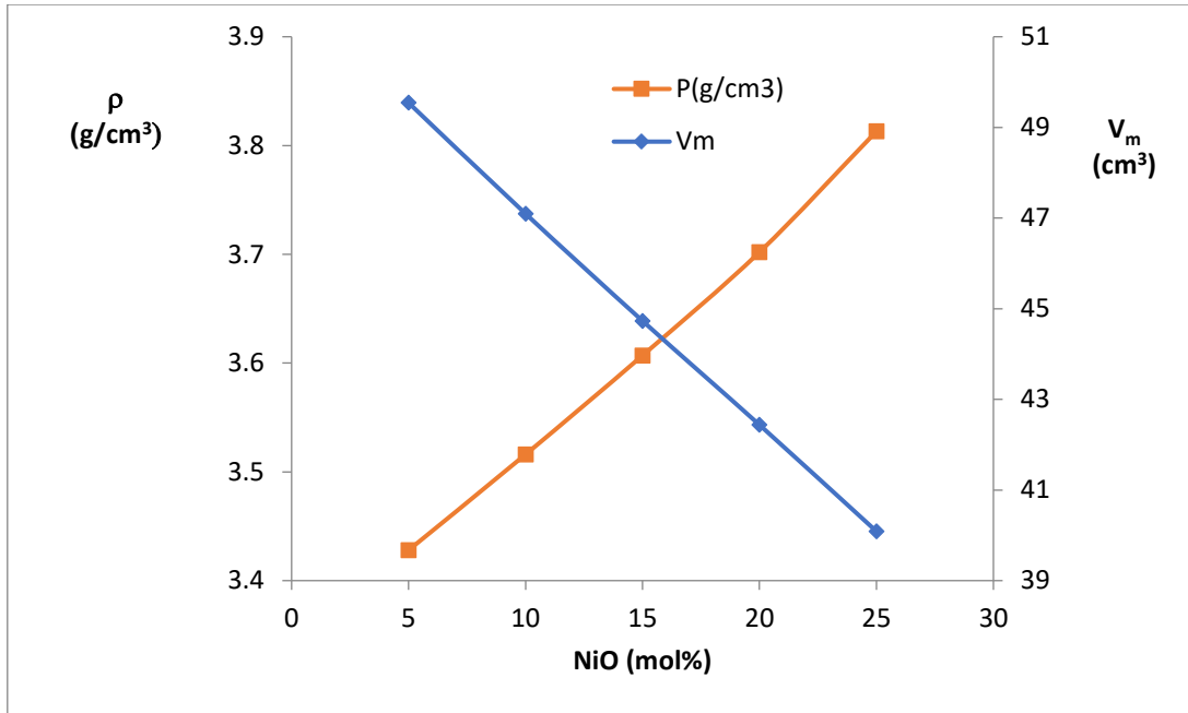
Fig. 3: Composition dependence of density ( \rho ) and molar volume ( V_m ) on NiO (mol%) contents.
