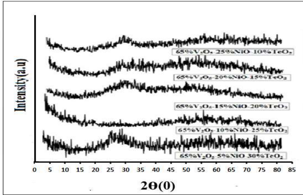
Fig.2: XRD patterns for V_2O_5 -NiO- TeO_2 glass of different compositions.
