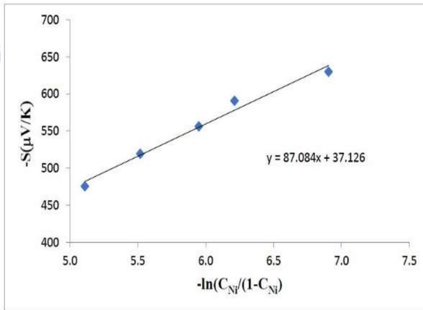
Fig. 6: Relationship between -S ( \mu\text{V}/\text{K} ) and [\ln(C/(1-C))] for the five 65V 2 O 5 -NiO-TeO 2 glass compositions.
