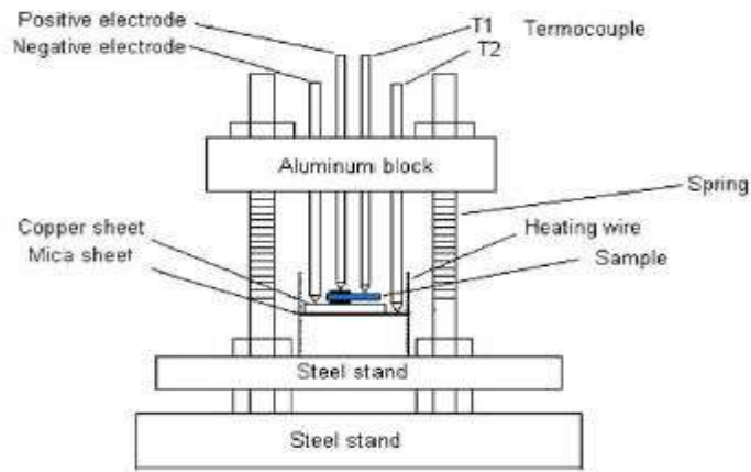
Fig. 1: shows the sample holder's schematic diagram for thermoelectric power measurements.
