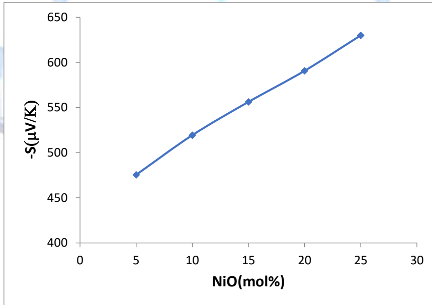
Fig. 5: Variation of the Seebeck coefficient with V2O5-NiO- TeO_2 glass.
