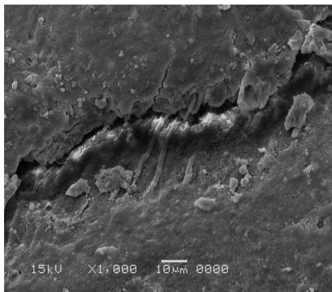
Figure 7-II: SEM photomicrograph of resin/dentin interface of oblique technique showing a thin hybrid layer with many long resin tags with small continuous gaps along the interface.
