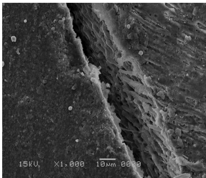
Figure 7-I: SEM photomicrograph of resin/dentin interface of bulk placement group showing a thin hybrid layer, long and ruptured dentin resin tags arranged perpendicular to the interface with continuous gaps along the interface.
