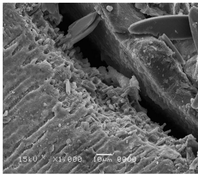
Figure 7-IV: SEM photomicrograph of resin/dentin interface of vertical placement, showing a non-uniform hybrid layer, with short, thin resin tags extending a small distance into dentinal tubules with gap formation along the interface.
