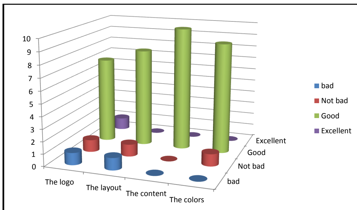
Figure 1: The graphic representation for the fifth question results about rank of LJD.
