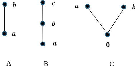
Fig. 1. Counter models for propositional formulas
