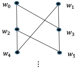
Fig. 2. The generic Kripke model R_1
