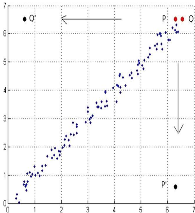
Fig.1. The different circumstances on the rectangle [0, 2\pi] \times [0, 2\pi] and the torus (from Zhan et al., 2019).
