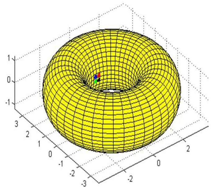
Fig.1. The different circumstances on the rectangle [0, 2\pi] \times [0, 2\pi] and the torus (from Zhan et al., 2019).
