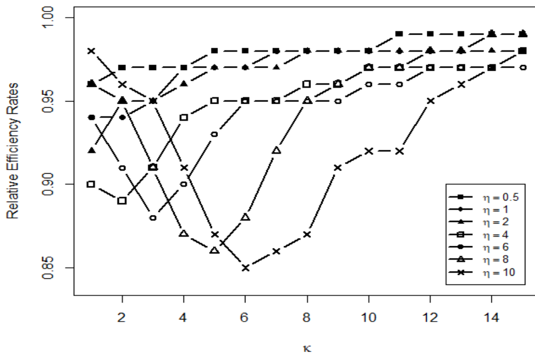
Fig 2. The efficiency rates of estimation based on MPL method compared to estimation based on ML method for the bivariate von Mises sine torus distribution with \kappa_1 = \kappa_2 = \kappa = 1, 2, \dots, 15 and \eta = 0.5, 1, 2, 4, 6, 8, 10 .
