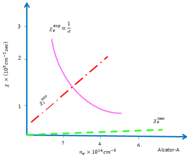
Fig. 3. Alcator (A) experimental results
