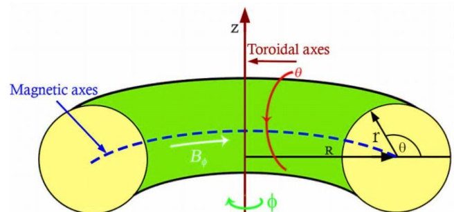
Fig.1. Toroidal tokamak coordinates
