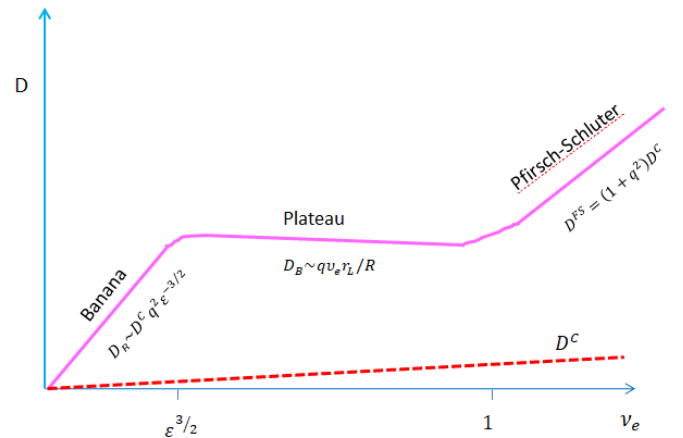
Fig.3. Transport diffusion coefficients
