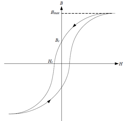
Fig. 3: Magnetizing Curve for a Soft Magnetic Material.
