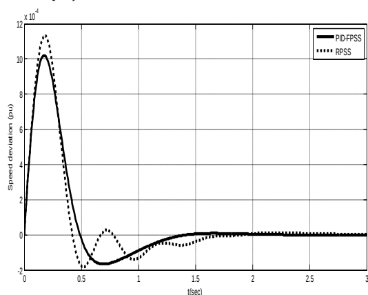
Fig. (5): Speed deviation response at ( P_e = 0.8 pu).
