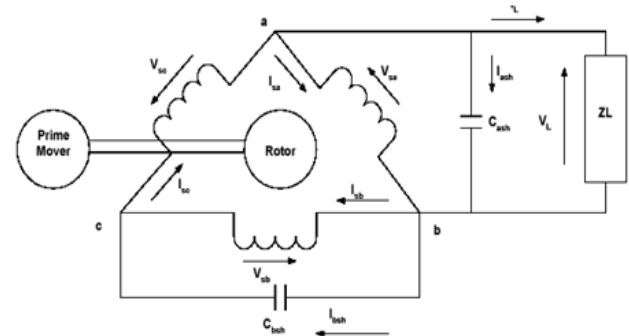
Figure 5: Connection of Self Excited Induction Generator of C-2C Scheme.
