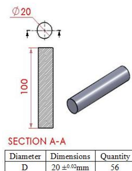
Fig. 1: Electrode design.
