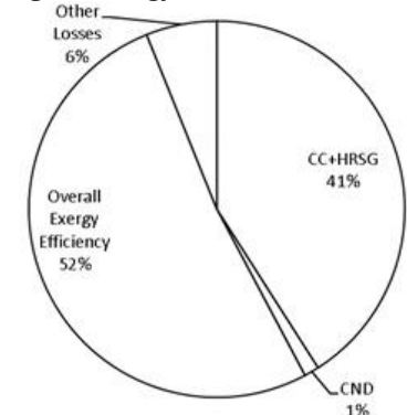
Fig. 5: Exergy balance of the CCPP.
