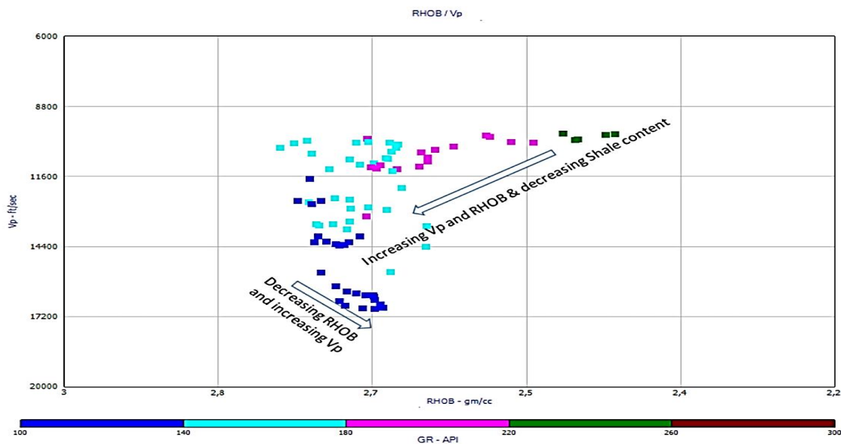
Figure 11. Cross plot of velocity versus grain density indicating a decrease in shale content as Velocity and density increases and apppoint of reversal in density as velocity slightly increases
