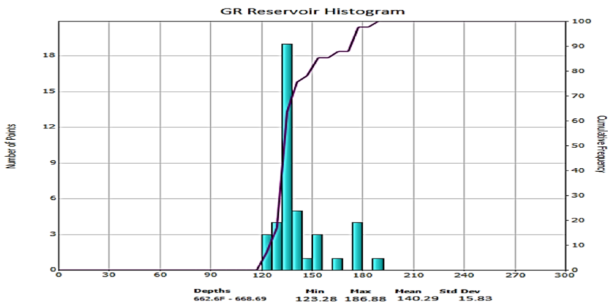
Figure 12. Histogram plot of GR showing limits (minimum, mean and maximum values) used for calculation of the volume of clay.
