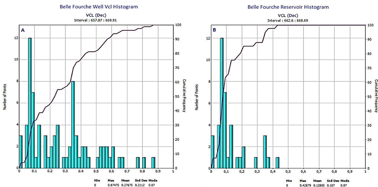
Figure 3. Histogram of (a) well volume of clay and (b) reservoir volume of clay.
