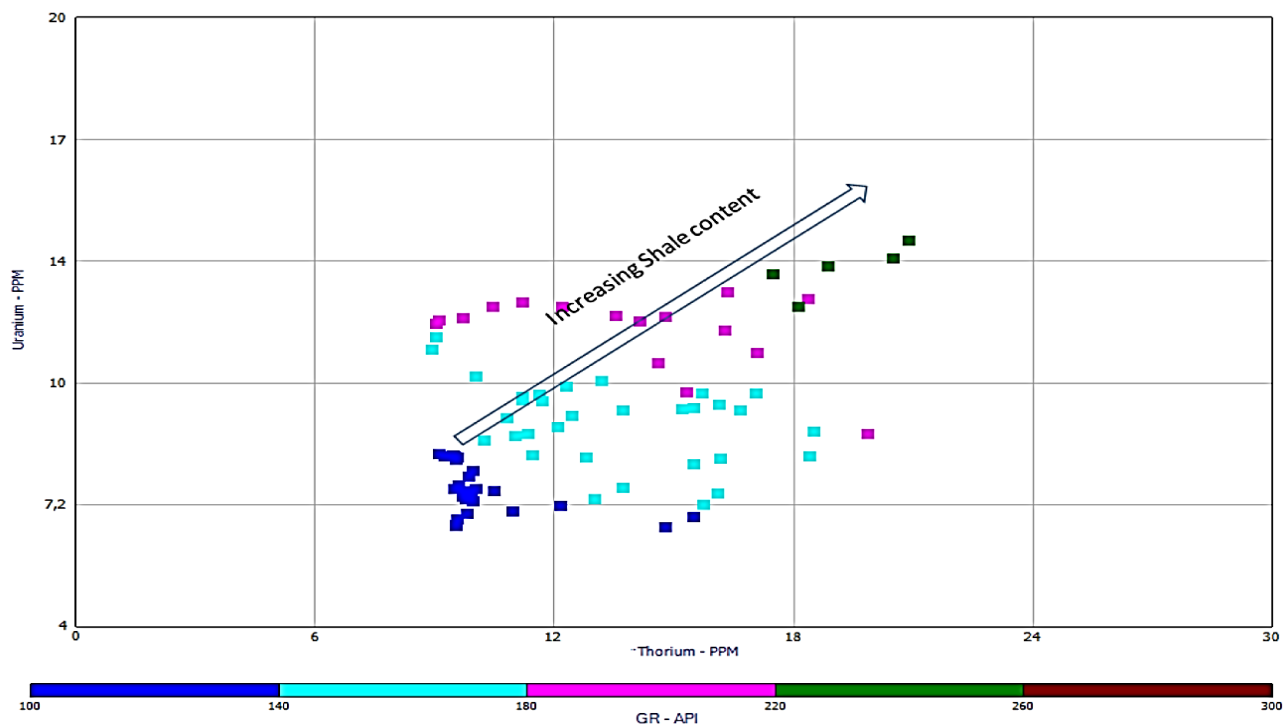
Figure 9. Cross plot of Uranium Versus Thorium indicating increasing shale content as the concentration of uranium and Thorium increases.
