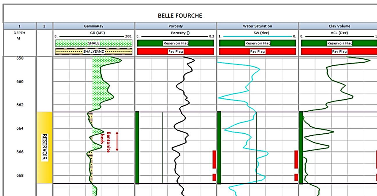
Figure 14. Results of final petrophysical interpretation showing petrophysical properties and gross and net pay flags.
