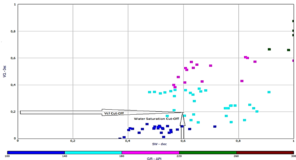
Figure 15: Cross plot of the volume of clay versus water saturation showing cut-off point
