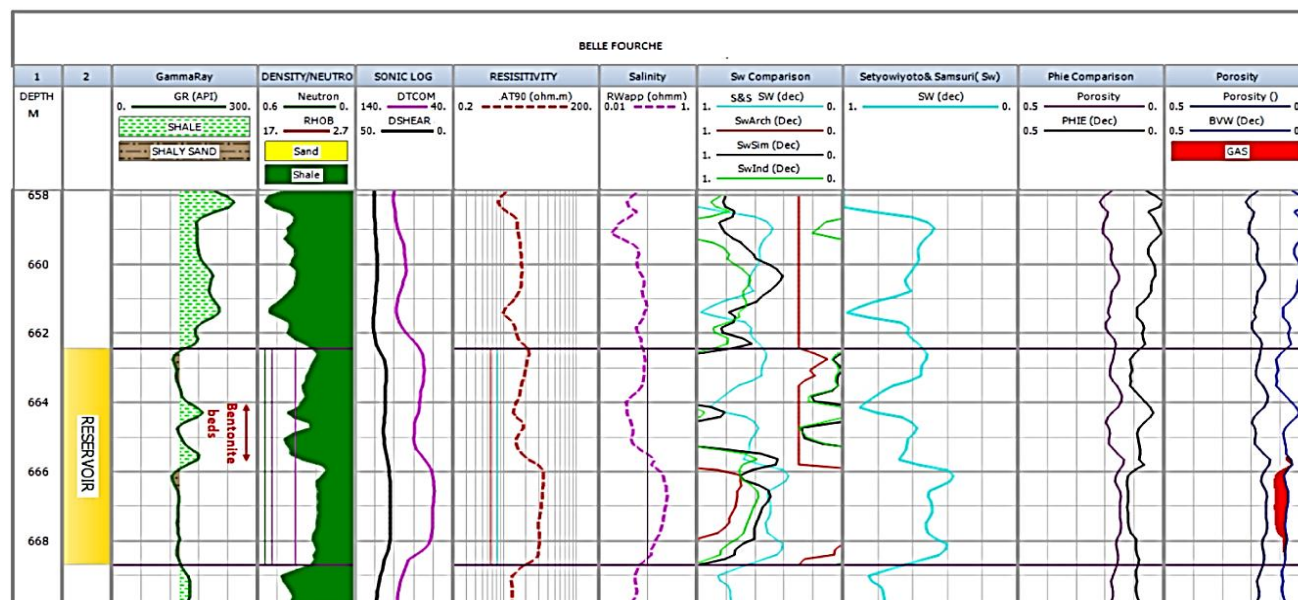
Figure 13. Results of basic log analysis showing reservoir interval and logs used for petrophysical evaluations.
