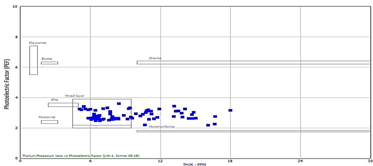
Figure 10. Cross plot of PEF log versus TH/K ratio to identify lithology showing the concentration of mixed clay minerals and montmorillonite.
