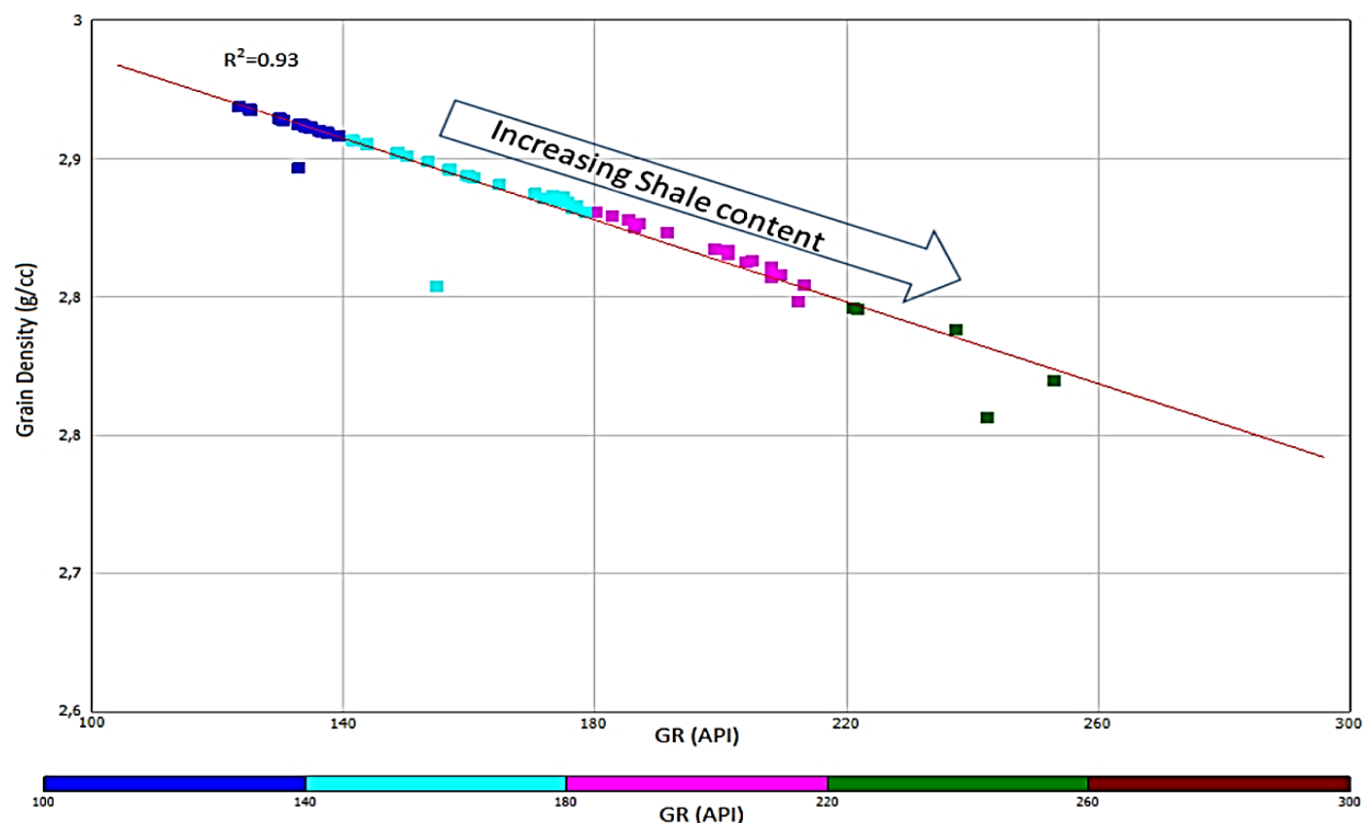
Figure 6: Cross plot of Grain density versus GR log for the identification of lithology.
