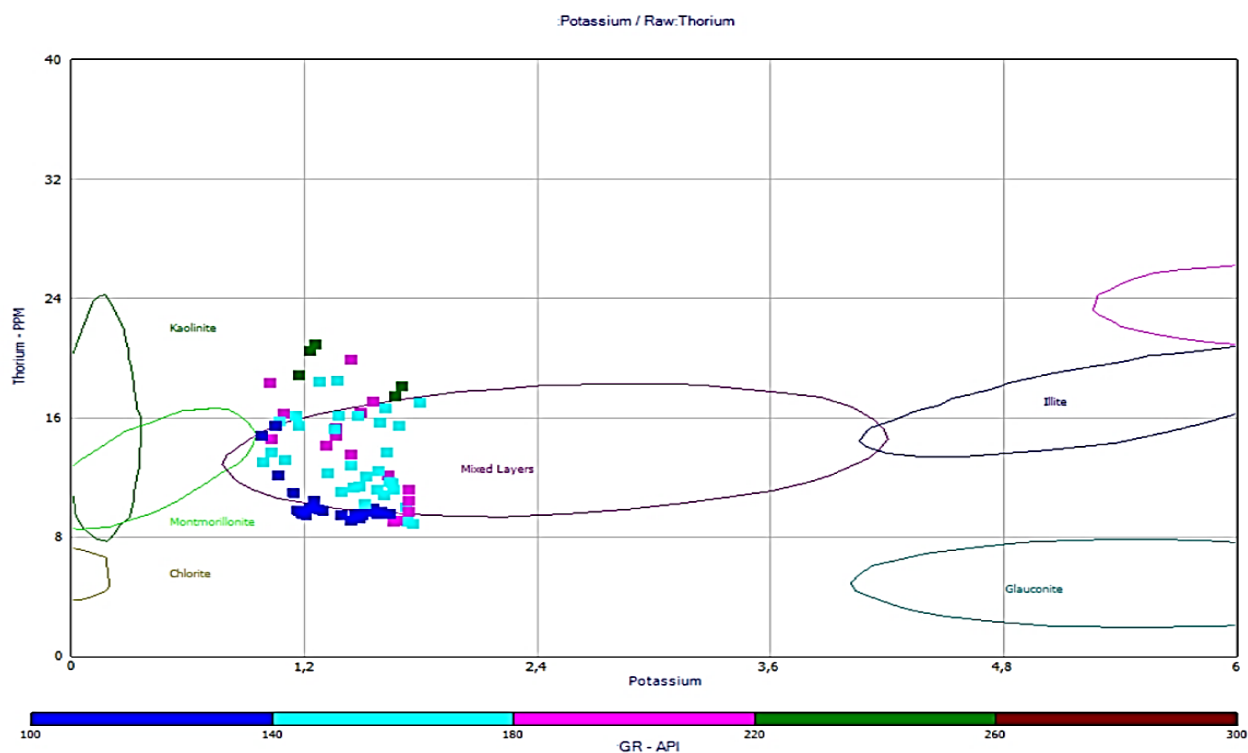
Figure 8b. Cross plot of Thorium Versus Potassium showing the concentration of mixed clay minerals.
