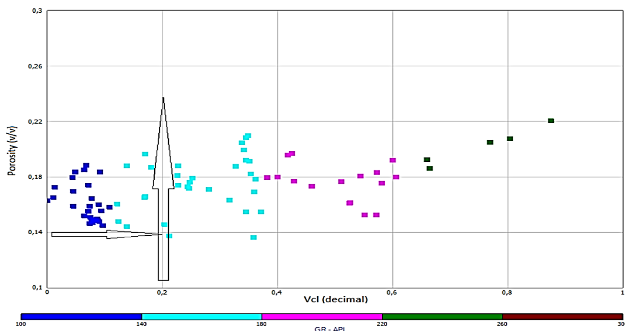
Figure 16: Cross plot of Porosity versus volume of clay showing cut-off points of 14 and 20 percent.
