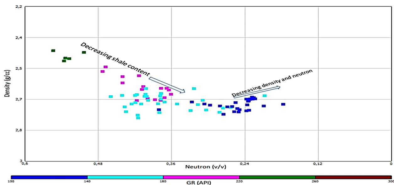
Figure 7: Cross plot of Density (RHOB) versus Neutron log for the identification of lithology.
