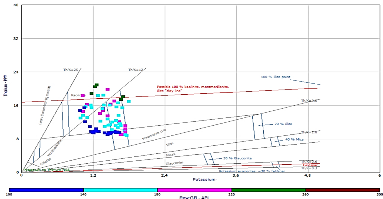
Figure 8a. Cross plot of Thorium Versus Potassium, showing the concentration of mixed clay minerals.
