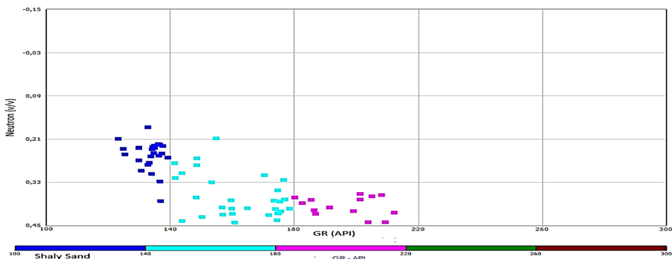
Figure 5: Cross plot of Neutron versus GR log for the identification of lithology.
