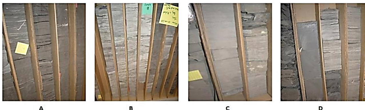
Figure 4. Core photographs of the study area. (a) Dark-grey calcareous shale & mudstone. (b) A uniform, greyish-black, non-calcareous shale low angle ripples interbedded with very fine sand & intercalated siltstone laminations. The coarsening-upward sequences form the main reservoir in the upper part of the BF. (c) Shaly silt with calcite cemented in the lower portion of the BF. (d) A sharp contact separates the cemented shaly-sand with dark shale. Bioturbation increases of the shale traces are hard to see at the bottom.
