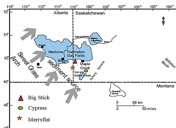
Figure 1. General map of Belle Fourche (Second White Specks sandstone), Hatton Gas Field [11]
