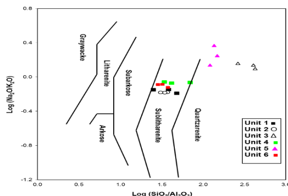
Fig.3. Chemical classification of the Mamuniyat Formation sandstones using \log(\text{SiO}_2/\text{Al}_2\text{O}_3) - \log(\text{Na}_2\text{O}/\text{K}_2\text{O}) diagram 5 .
