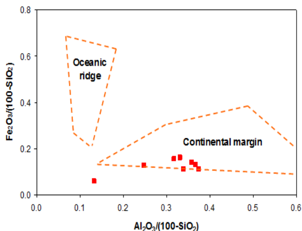
Figure 19: Binary plot of \text{Al}_2\text{O}_3/(100-\text{SiO}_2) vs. \text{Fe}_2\text{O}_3/(100-\text{SiO}_2) showing the paleotectonic setting for the studied sediments (fields after [32]).
