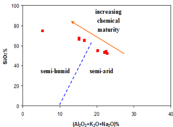
Figure 18: Binary plot of (\text{Al}_2\text{O}_3+\text{K}_2\text{O}+\text{Na}_2\text{O}) vs. \text{SiO}_2 showing the paleoclimate conditions for the studied sediments (fields after [30]).
