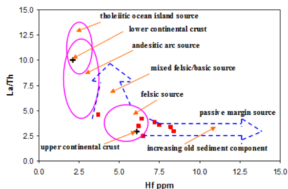
Figure 12. Binary plot of Hf vs. La/Th showing the provenance of the studied sediments (fields after [19]).
