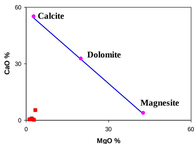
Figure 9. Binary plot of MgO vs. CaO showing the carbonate minerals in the studied samples (fields after [13]).
