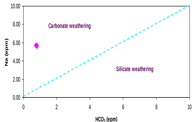
Figure 3: The plot of Na vs. \text{HCO}_3 of the water samples (field after 3 ).
