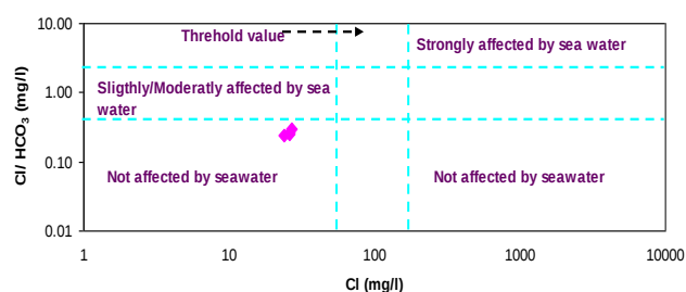
Figure 7: Molar ratio \text{Cl} vs. \text{Cl}/\text{HCO}_3 in the water samples (fields after 6 ).
