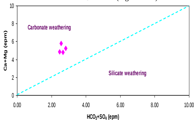
Figure 2: Plot of \text{Ca} + \text{Mg} vs. \text{HCO}_3 + \text{SO}_4 of the water samples (field after 3 ).
