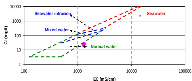
Figure 8: Molar ratio EC vs. \text{Cl} in the water samples (fields after 6 ).
