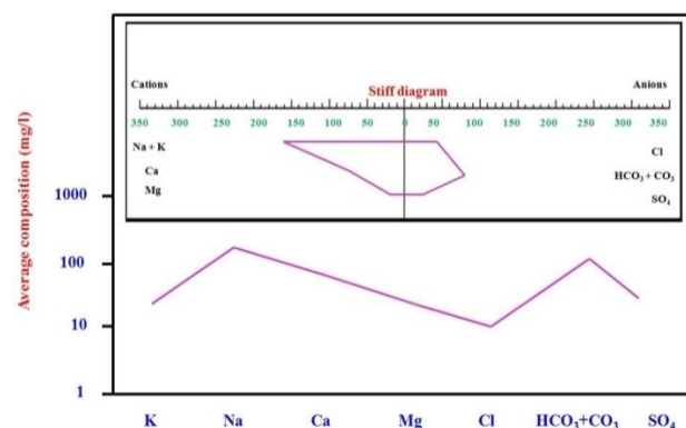
Figure 9: Schoeller diagram showing average composition in mg/l of the studied water samples. Stiff diagram is shown in inset 9 .
