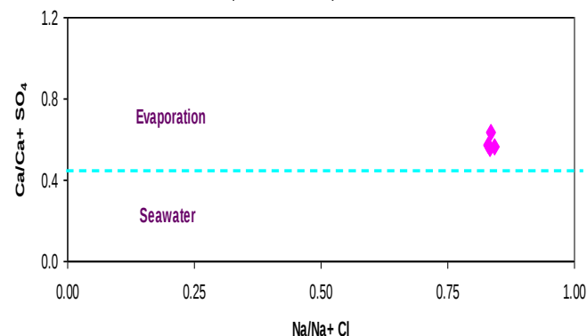
Figure 4: Molar \text{Na}/\text{Na}+\text{Cl} and \text{Ca}/\text{Ca}+\text{SO}_4 to differentiate water of different origin (field after 4 ).
