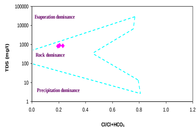
Figure 5: Dominance of rock precipitation and evaporation on \text{Cl}/\text{Cl}+\text{HCO}_3 vs. TDS of the studied water (field after 5 ).
