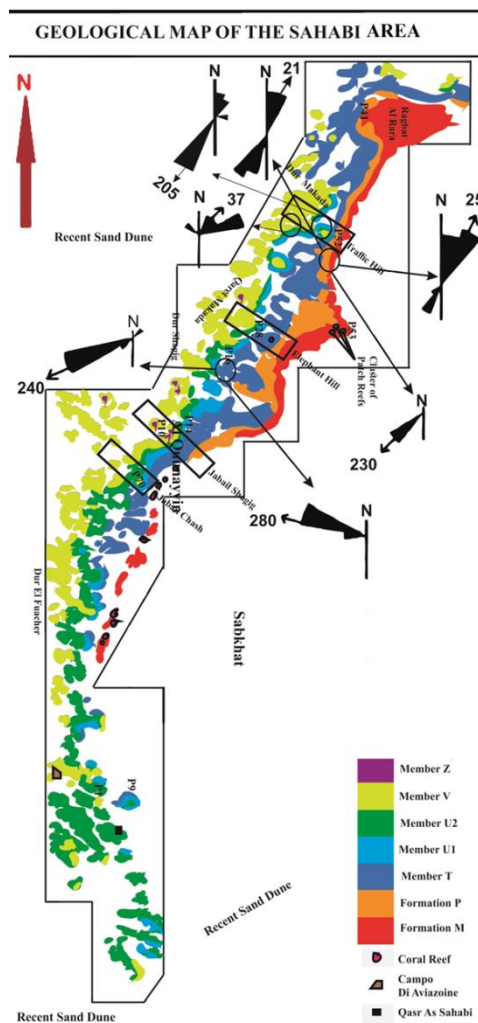
Figure 9. Geological map of the Sahabi area showing the studied stations and their paleocurrent directions and mean current. (Modified from de Heinzelin and El-Arnauti [25]).
