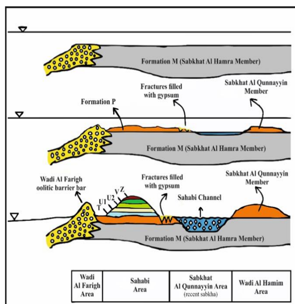
Figure 13. Schematic diagram showing stages of the depositional environments in the Wadi Al Farigh and As-Sahabi areas (not to scale).
