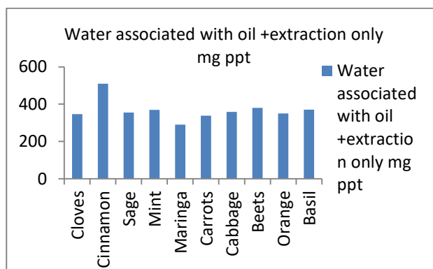
Figure 14. Shows the weight of metal ions precipitate in milligrams of water accompanied with oil with natural extractions by direct weight method.
