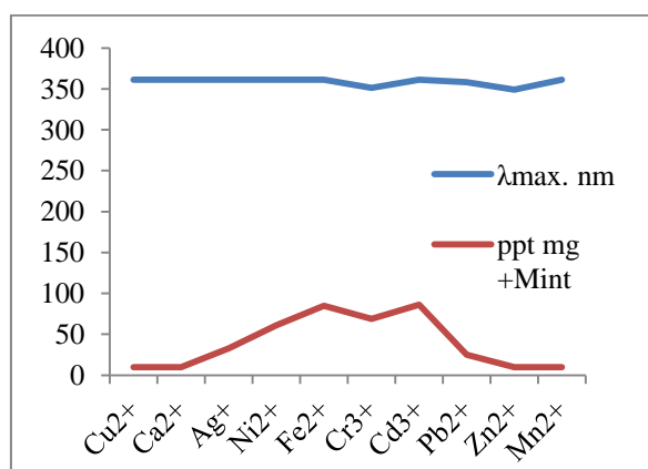
Figure 20. Shows the weight of metal ions precipitate in milligrams with Mint and corresponding maximum wavelength \lambda_{max} of filtrate.
