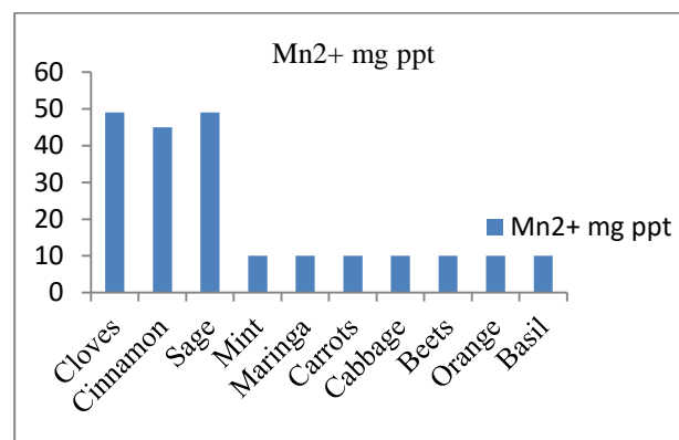
Figure 10. Shows the weight precipitate in milligrams of Manganese complexes which may be formed by adding 10 ml of extract to 10 ml of 0.1M Mn SO 4 . H 2 O.
