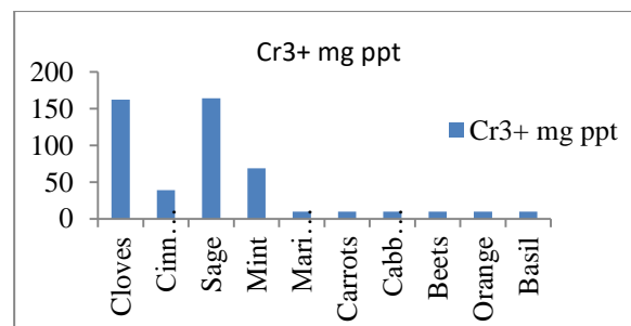
Figure 6. Shows the weight precipitate in milligrams of Chromium complexes which may be formed by adding 10 ml of extract to 10 ml of 0.1M Cr (NO 3 ) 3 .9H 2 O.
