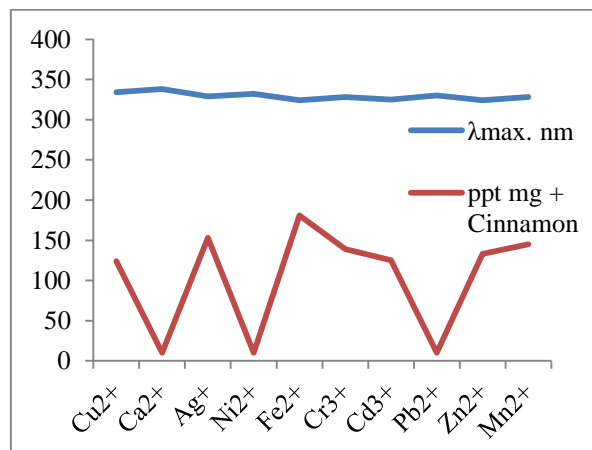
Figure 18. Shows the weight of metal ions precipitate in milligrams with Cinnamon and corresponding maximum wavelength \lambda_{max} of filtrate.
