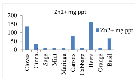
Figure 9. Shows the weight precipitate in milligrams of Zinc complexes which may be formed by adding 10 ml of extract to 10 ml of 0.1M ZnSO 4 .7H 2 O.
