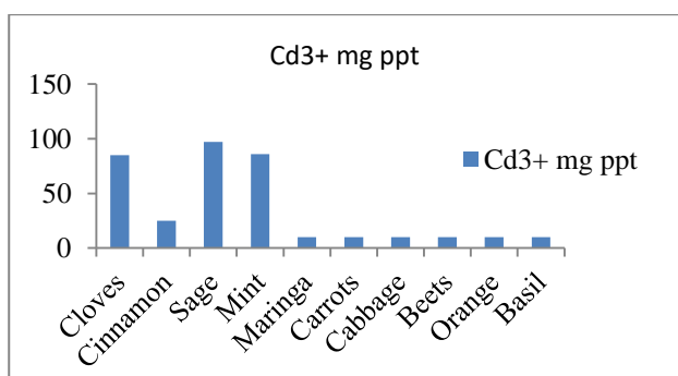
Figure 7. Shows the weight precipitate in milligrams of Cadmium complexes which may be formed by adding 10 ml of extract to 10 ml of 0.1M Cd (NO 3 ) 3 .4H 2 O.
