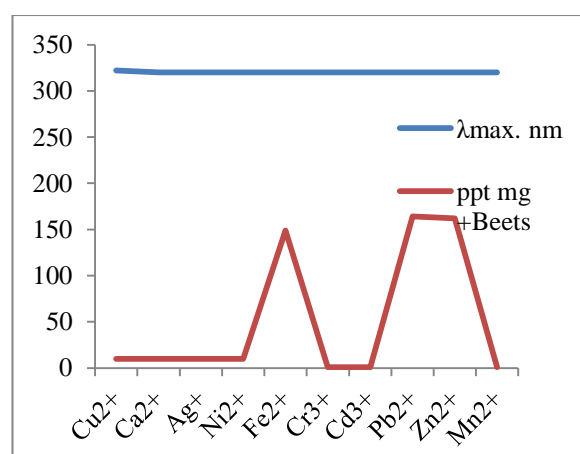
Figure 24. Shows the weight of metal ions precipitate in milligrams with Beets and corresponding maximum wavelength \lambda_{max} of filtrate.
