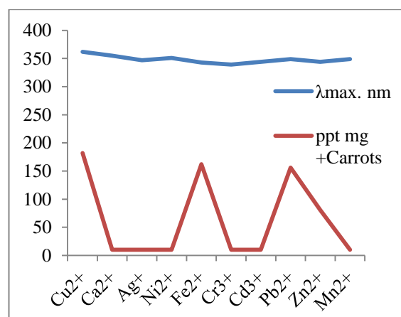
Figure 22. Shows the weight of metal ions precipitate in milligrams with Carrots and corresponding maximum wavelength \lambda_{max} of filtrate.
