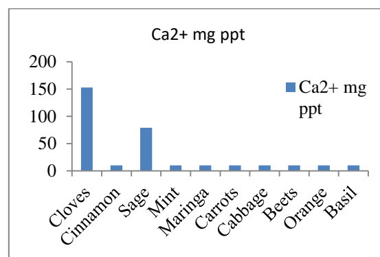
Figure 2. Shows the weight precipitate in milligrams of Calcium complexes which may be formed by adding 10 ml of extract to 10 ml of 0.1M Ca (NO 3 ) 2 . 4H 2 O.
