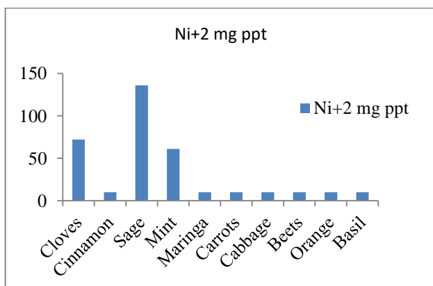
Figure 4. Shows the weight precipitate in milligrams of Nickel complexes which may be formed by adding 10 ml of extract to 10 ml of 0.1M NiCl 2 .6H 2 O.
