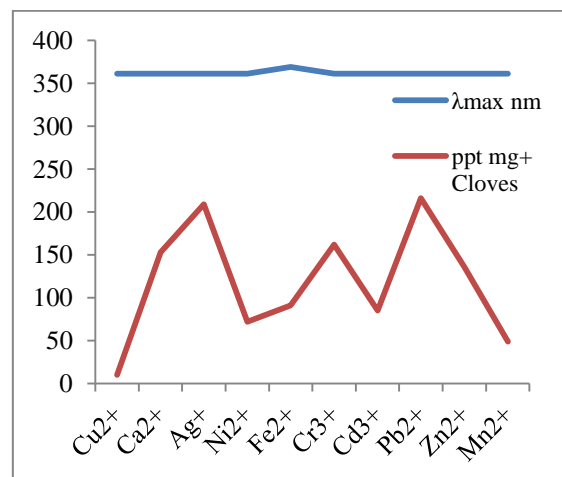
Figure 17. Shows the weight of metal ions precipitate in milligrams with Cloves and corresponding maximum wavelength \lambda_{max} of filtrate.
