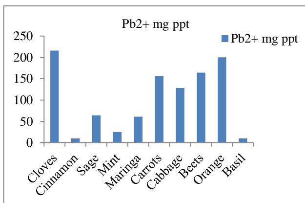
Figure 8. Shows the weight precipitate in milligrams of Lead complexes which may be formed by adding 10 ml of extract to 10 ml of 0.1M (CH 3 COO) 2 Pb 3H 2 O.
