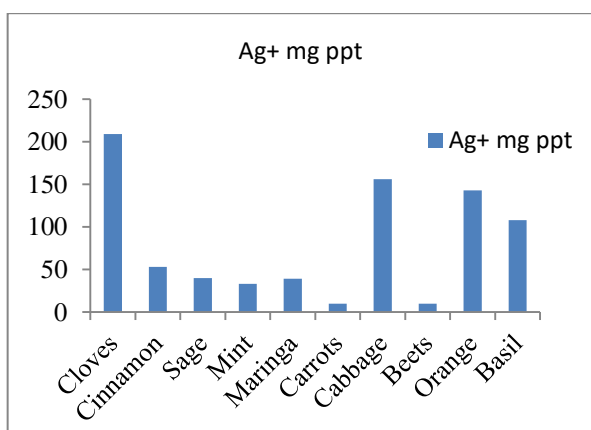
Figure 3. Shows the weight precipitate in milligrams of silver complexes which may be formed by adding 10 ml of extract to 10 ml of 0.1M AgNO 3 .
