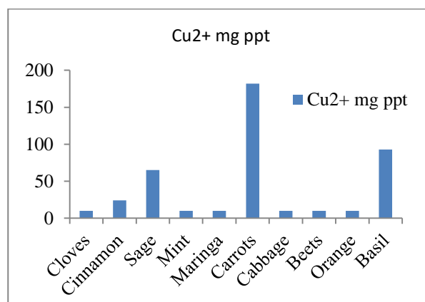
Figure 1. Shows the weight precipitate in milligrams of copper complexes which may be formed by adding 10 ml of extract to 10 ml of 0.1M Cu SO 4 .5H 2 O.
