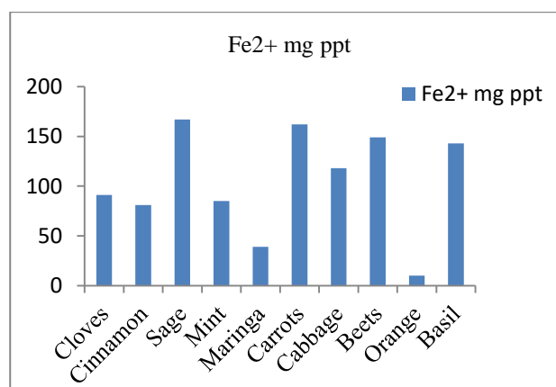
Figure 5. Shows the weight precipitate in milligrams of Ferrous complexes which may be formed by adding 10 ml of extract to 10 ml of 0.1M Fe SO 4 .7H 2 O.
