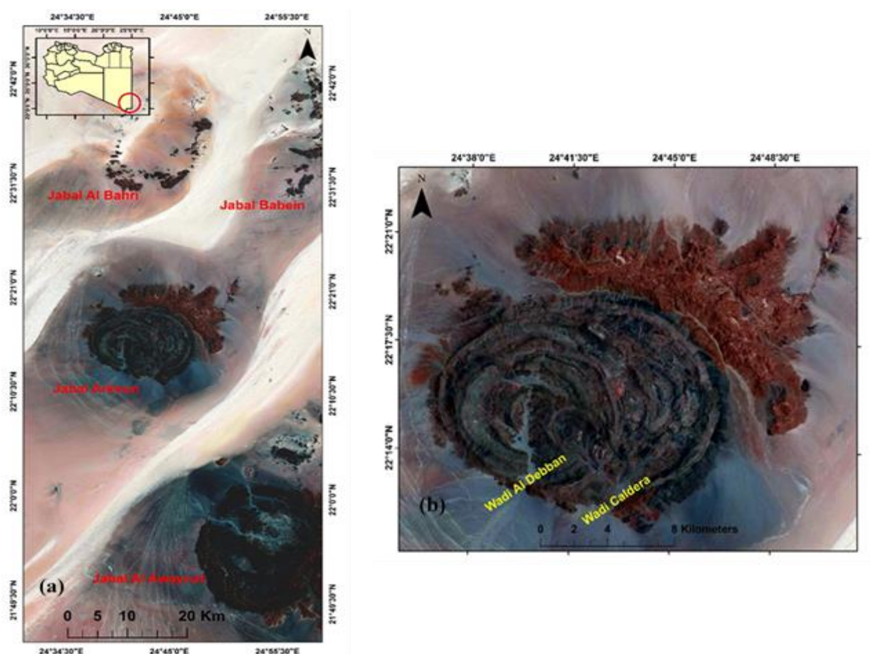
Figure. 1. a) General location of the study area and a satellite image showing Jabal Al Awaynat, Jabal Arkeun, Jabal Al Bahir and Jabal Babein; b) Satellite image of Jabal Arkenu Ring Complex.
