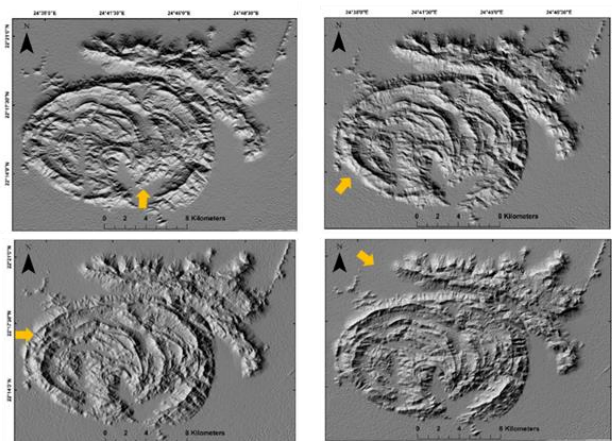
Figure.5. Shows the second four shaded relief images derived from simulating the sunlight in four azimuth directions (180, 225, 270, & 315); the yellow arrows represent the direction of applied light on the DEM.
