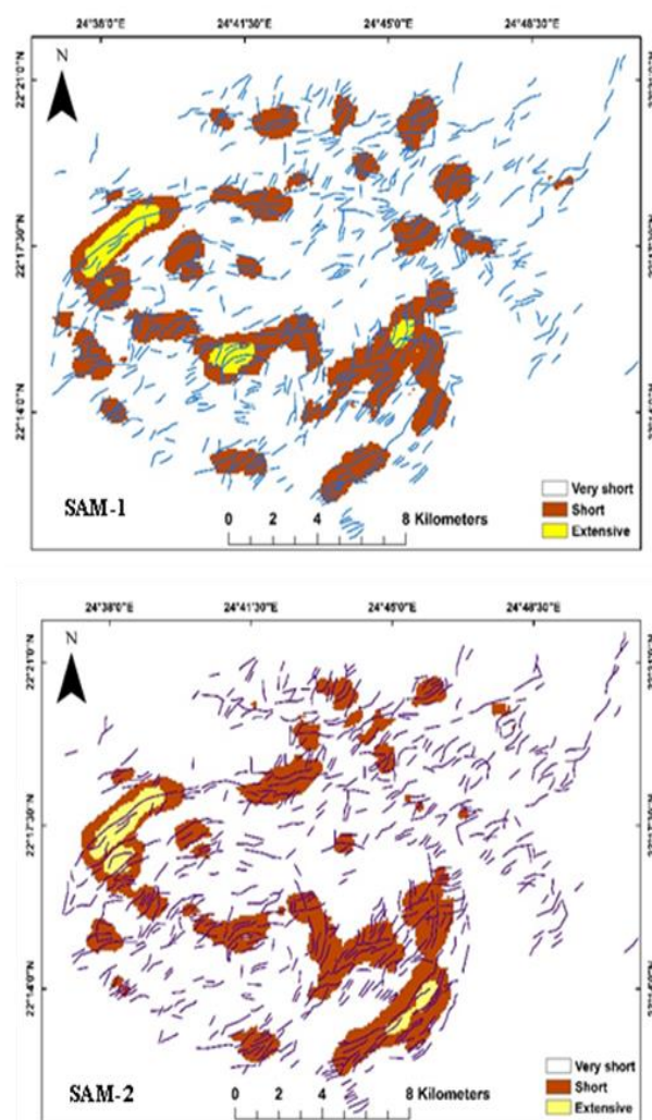
Figure.9. Shows the length maps lineament of SAM-1 and SAM-2.
