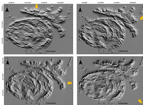
Figure 4. Shows the first four shaded relief images derived from simulating the sunlight in four azimuth directions (0, 45, 90, & 135); the yellow arrows represent the direction of applied light on the DEM.
