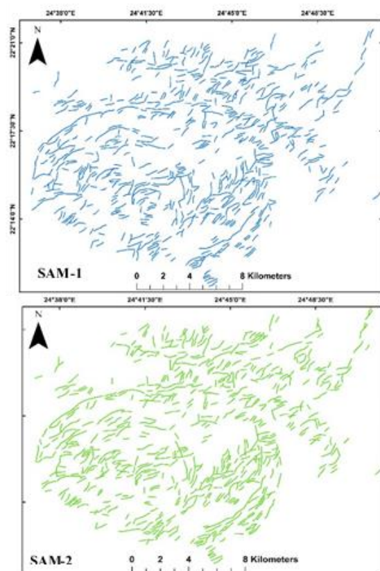
Fig.7 Two lineament maps of shaded relief images by PCI Geomatica.
