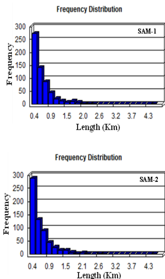
Figure. 8. Two frequency distributions of automatic extraction lineaments.
