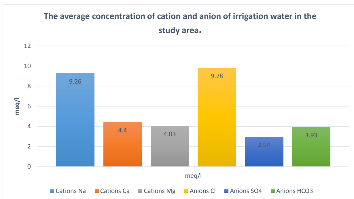
Figure 2: The average concentration of cation and anion of irrigation water in the study area.
