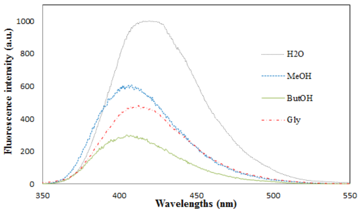
Fig 4. Dependence of fluorescence excitation of AmNS-ALG on solvent polarity. Equal amounts of AmNS-ALG (10-1 wt%) were taken in water (H 2 O), methanol (MeOH), butanol (ButOH), and glycerol (Gly) and in the fluorescence excitation Scanned for each sample.
