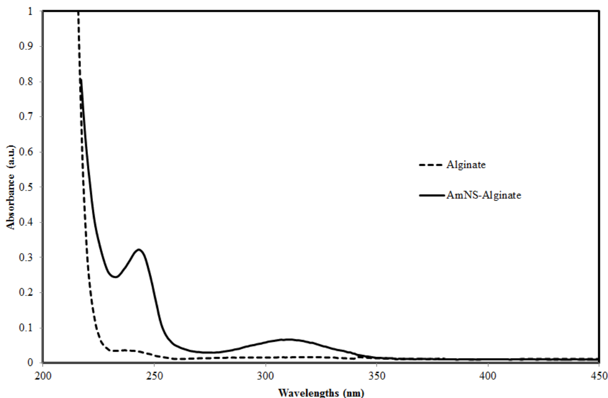
Fig 1. UV-Absorption spectra of 10-1 wt% AmNS-labelled alginate and alginate
