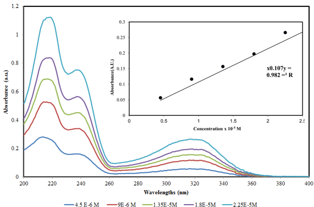
Fig 2. Beer-Lambert's law of AmNS at different molar concentrations in an alcoholic solution. ( \lambda_{\text{max}} = 320 \text{ nm} )
