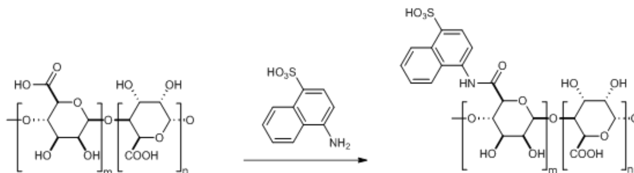
Scheme 1. Chemical structure of AmNS-labelled alginate, where n is significantly larger than m .
