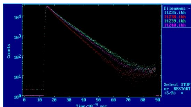
Figure 5. Fluorescence decay lifetimes of AmNS in different solvents.
