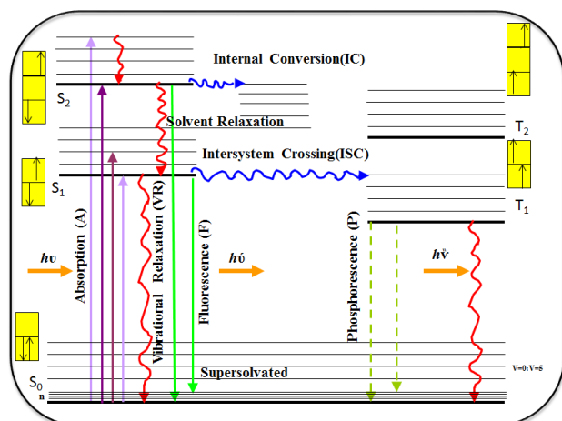
Scheme 2. A Jablonski transition state diagram showing solvent relaxation and intersystem crossing.
