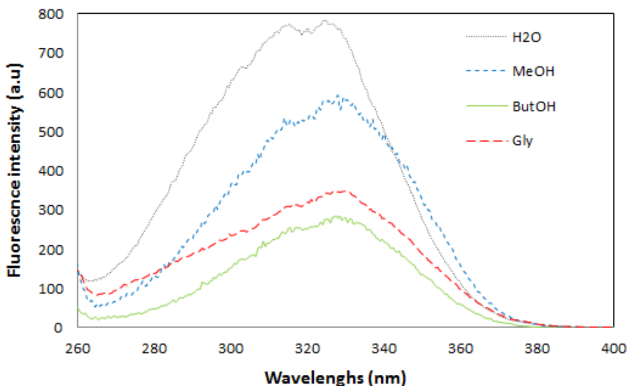
Fig 3. Dependence of fluorescence excitation of AmNS-ALG on solvent polarity. Equal amounts of AmNS-ALG (10-1 wt%) were taken in water (H 2 O), methanol (MeOH), butanol (ButOH), and glycerol (Gly) and in the fluorescence excitation Scanned for each sample.
