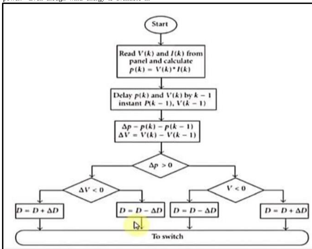
Figure. 5. Flowchart of MPPT algorithm wind turbine for the boost converter [8]
