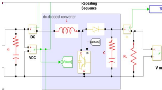
Figure.4. DC-DC boost converter.
