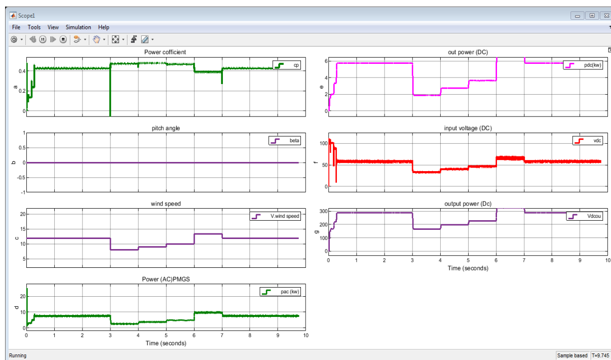
Figure 6. Simulation results: (a) shows the power coefficient,(b) The pitch angle control (c) shows the variable wind speed,(d) shows the power of the alternating current in PMSG,(e) shows the output power,(f) shows the input voltage of the Dk8C,(g) shows the output voltage of the DC.
