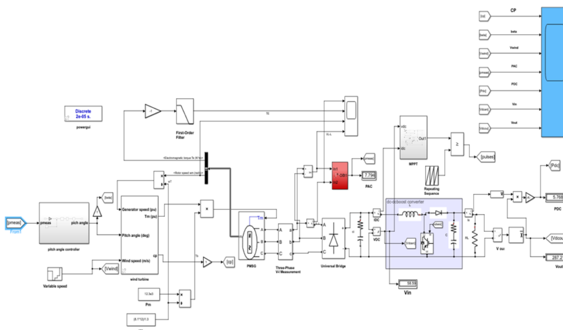
Figure.1. modeling of a wind energy conversion system considering variable wind speed.
