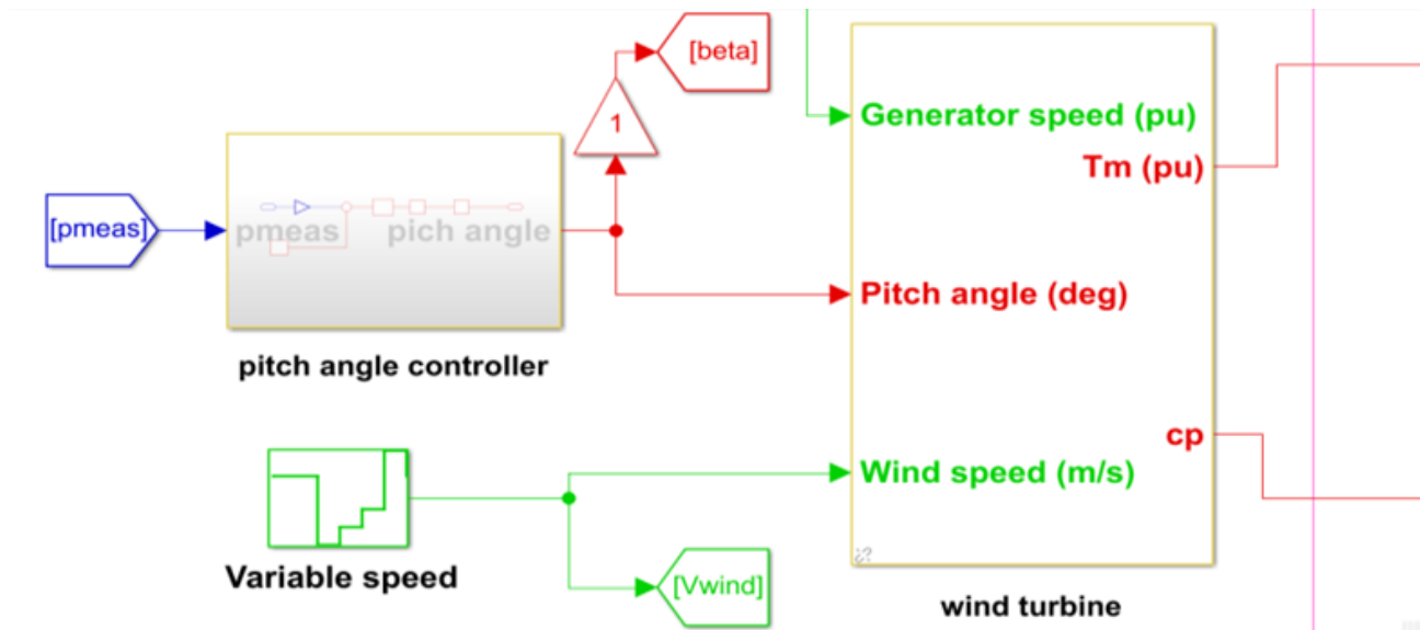
Figure. 2. wind turbine
