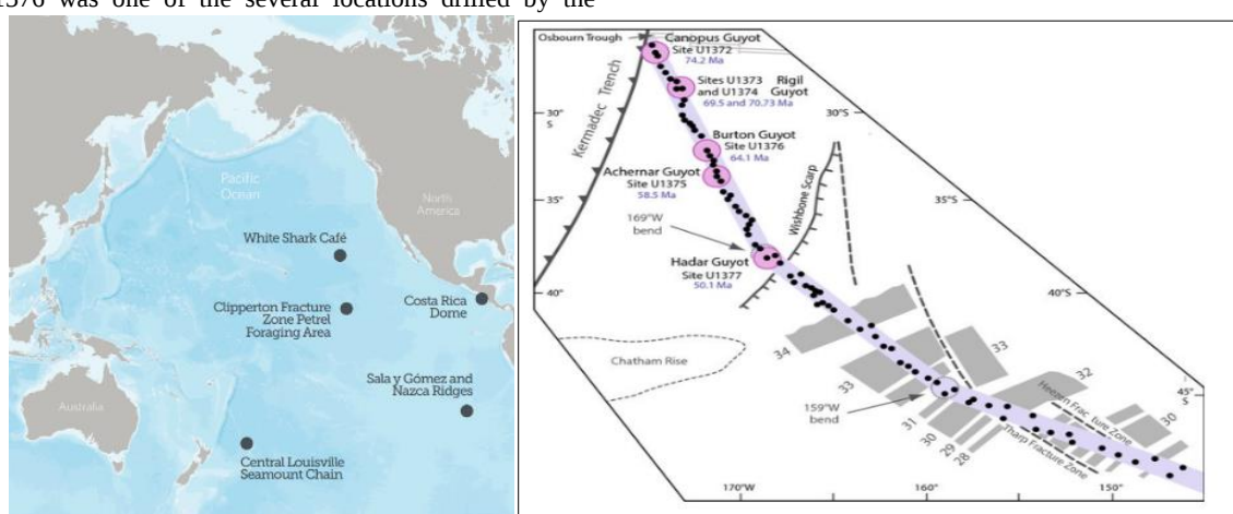
Figure 1. Location and age in millions of years of the Burton Guyot, which was drilled by IODP Expedition 330 along the Louisville Seamount Chain [8,9].
