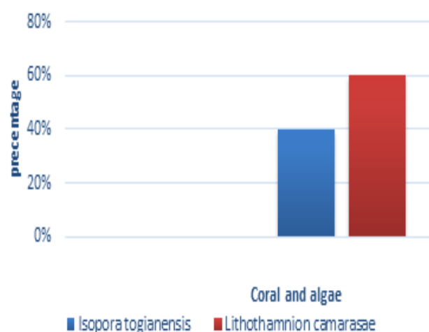
Figure 6a. Histogram showing the distribution of the coral ( Isopora togianensis ) against the red algae ( Lithothamnion camarasae ) in the Algal Reef (Limestone Unit IIA).
