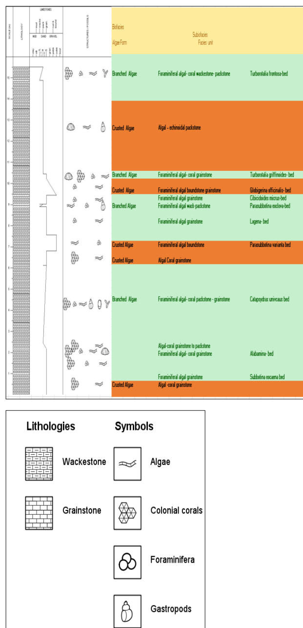
Figure 3. General description of the studied cored Limestone Unit IIA.
