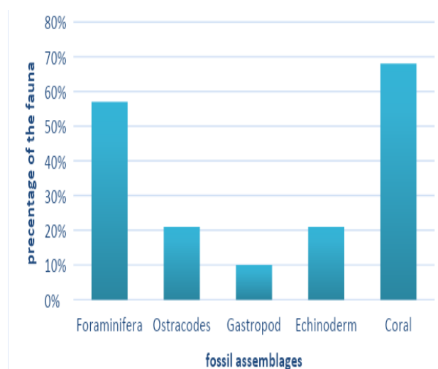
Figure 5. Histogram showing the distribution of the reported fossils in the algal reef (Limestone Unit IIA) in the thin sections.
