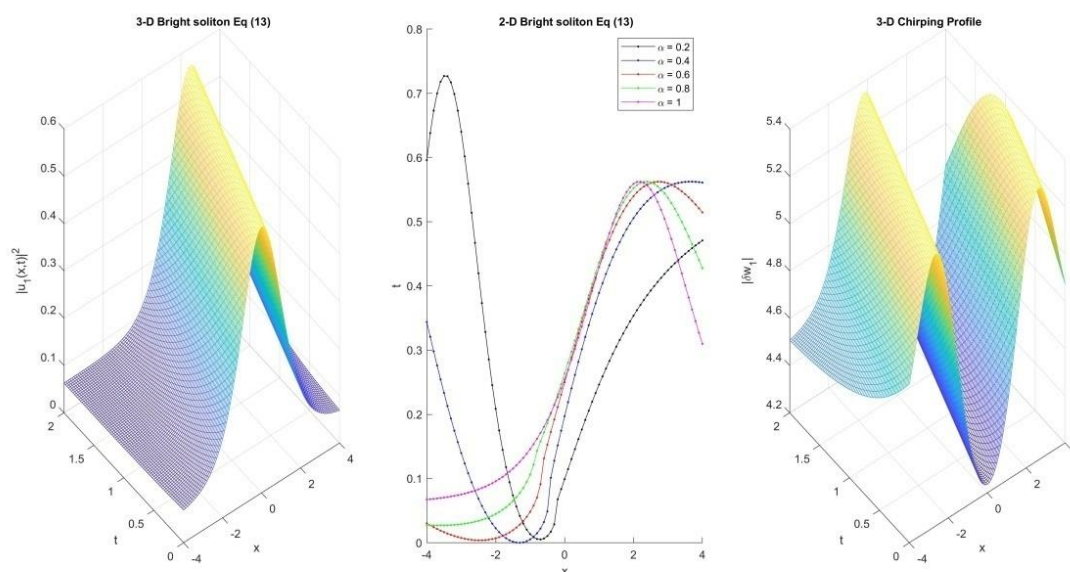
Figure 1: 3D, 2D and 3D chirped Bright soliton solutions of Equation (13) for a_1 = 0.15, a_2 = 0.5, a_3 = 2, b_0 = 0.25, \gamma = 0.5, b_1 = 1, C = 0.5 , and \alpha = 1 , with x \in [-4, 4] and x \in [0, 2] .
