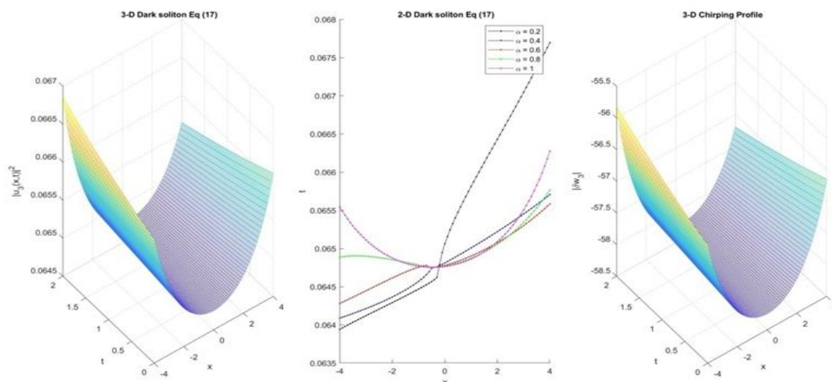
Figure 2: 3D, 2D and 3D chirped Dark soliton solutions of Equation (17) for \mathbf{a_1 = 0.15, a_2 = 0.05, a_3 = 0.2, b_0 = 0.25, \gamma = -0.05, b_1 = 0.02, C = 5,} and \alpha = 1 , with \mathbf{x \in [-4, 4]} and \mathbf{x \in [0, 2]} .
