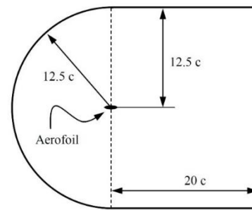
Fig. 1. Airfoil domain dimensions
