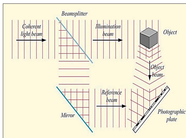
Figure 4: Recording a hologram.
