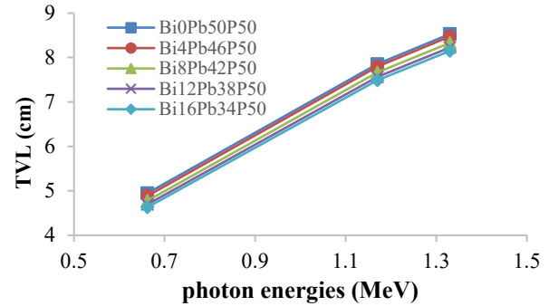
Fig 15: The relationship between tenth value layer (cm) and photon energy for \text{Bi}_2\text{O}_3\text{-PbO-P}_2\text{O}_5 glasses at different photon energies (theoretically).
