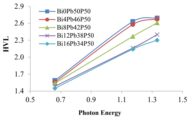
Fig 12: The relationship between half-value layer (cm) and photon energy for \text{Bi}_2\text{O}_3\text{-PbO-P}_2\text{O}_5 glasses at different photon energies (experimentally).
