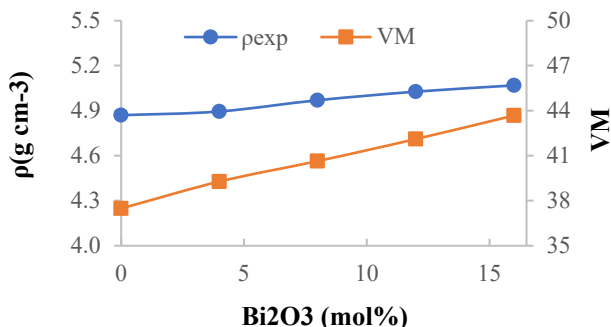
Fig 4: Variation of \rho_{exp} and V_M with Bi 2 O 3 mol% content.
