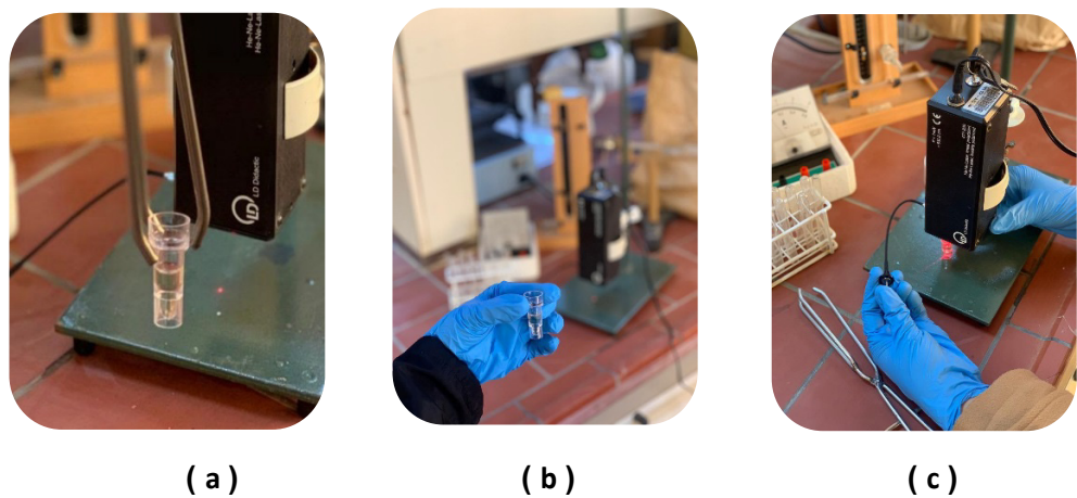
Figure (1) : Samples preparation and set up the helium-neon laser device. (a) Serum sample placed in a cuvette ready for laser irradiation. (b) Sample being manually prepared and positioned by the operator. (c) Fine adjustment of the He-Ne laser device to ensure accurate and uniform exposure.
