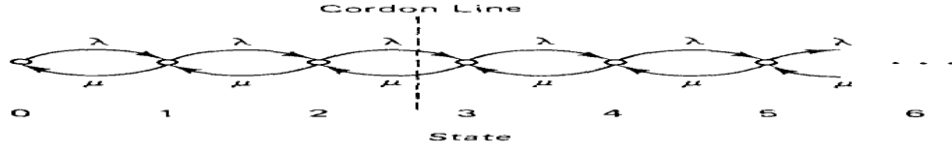
Figure 1 Transition rate diagram for the ( M/M/1):(GD/ ∞/ ∞ ) queue.
