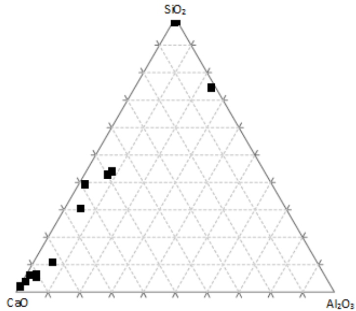
Figure (7) \text{SiO}_2 - \text{CaO} - \text{Al}_2\text{O}_3 Ternary plot showing the interbedded of limestone and sandstone rocks in Zallah area.
