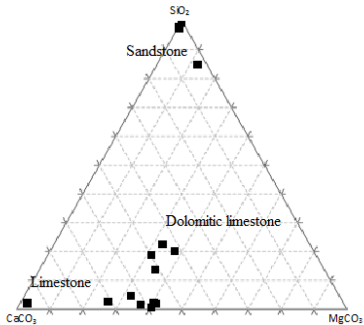
Figure (8) \text{SiO}_2 - \text{CaCO}_3 - \text{MgCO}_3 Ternary plot of the different carbonate rock types in Zallah area
