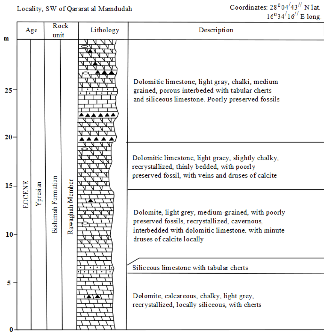
Figure (4) Columnar section of the Bishimah Formation (after Vesely, 1985).
