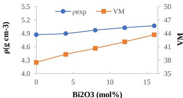
Fig 4: Variation of \rho_{\text{exp}} and V_M with \text{Bi}_2\text{O}_3 mol% content.
