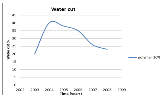
Figure 12: Water cut curve case (2), (with 10% of polymer).
