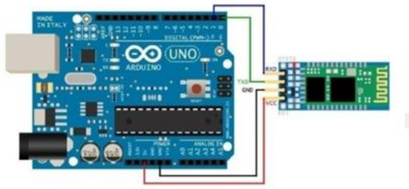
Fig. 13. Connection of the arduino with Bluetooth module.
