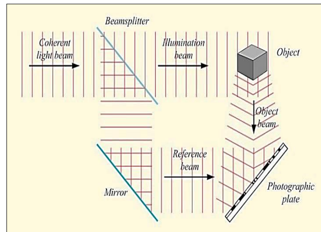
Figure 4: Recording a hologram.
