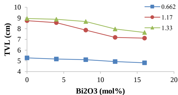
Fig 17: The relationship between tenth value layer (cm) and \text{Bi}_2\text{O}_3 (mol%) content for \text{Bi}_2\text{O}_3\text{-PbO-P}_2\text{O}_5 glasses (experimentally).
