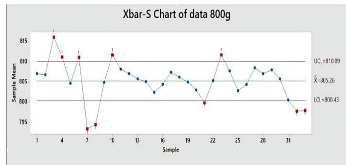
Figure 2. X-bar chart for Jam Filling Process.
