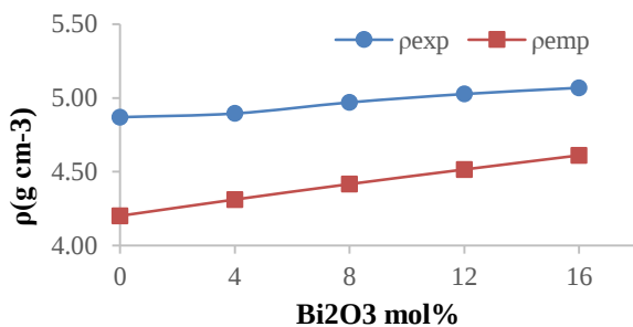
Fig 2: The experimental and empirical densities as a function of \text{Bi}_2\text{O}_3 mol% content.
