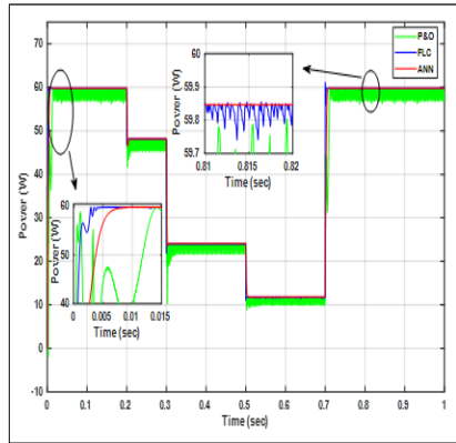
Figure. (21): Output power from P&O and ANN and FLC under varying irradiance conditions
