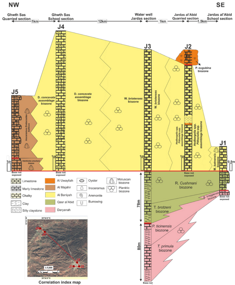
Figure. (9): Biostratigraphic correlation of the measured sections (J1–J5), illustrating the distribution of lithologic units and biostratigraphic zones across the study area. The correlation is referenced to the base of the Al Baniyah Formation (datum line). Note: the lower part of section J3 is presented at a different vertical scale.
